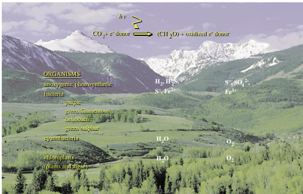
Figure 14. Photosynthesis and the generation of oxidants. This diagram is meant to illustrate that although photosynthesis does indeed result in the production of organic carbon ( \text{CH}_2\text{O} ), it also plays an important role in the generation of oxidants. On earth, we know of photosynthetic organisms that use the energy of light to produce oxidized forms of sulphur, iron and water. Without light, or without some other way of generating oxidants, it is not clear how complex life could evolve.
